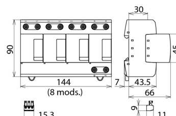
Dimension drawing DVA CSP 3P 100 FM
